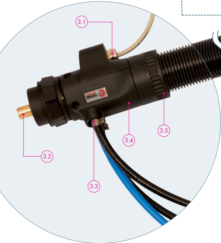
Fig. 3: Machine connection
